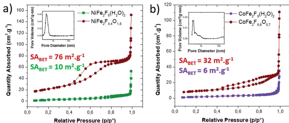
Fig. 4 N 2 adsorption/desorption isotherm of (a) NiFe 2 F 4.4 O 1.8 and (b) CoFe 2 F 6.6 O 0.7 before (green/purple) and after calcination (brown). Inset: corresponding BJH pore size distribution analyzed from the desorption branch.
