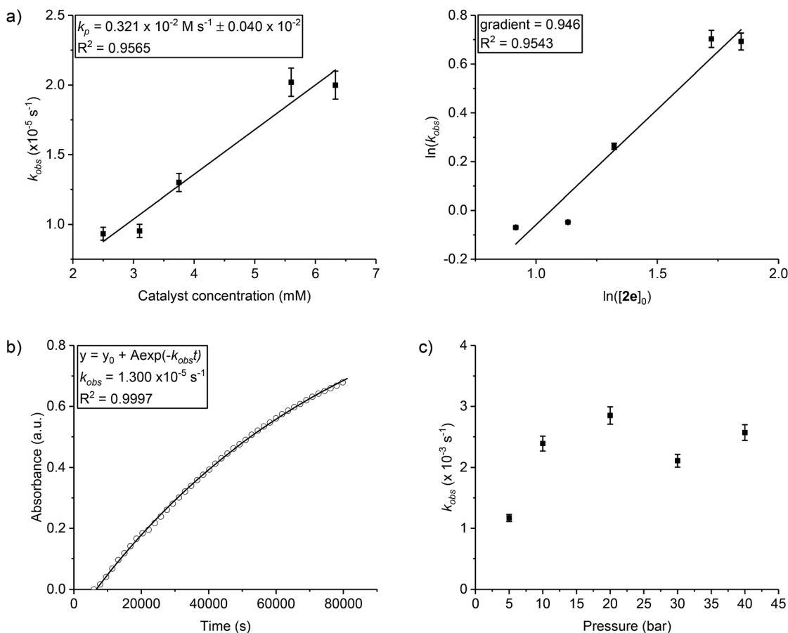
Fig. 1 Reaction kinetic analysis to determine order in (a) catalyst (first order); (b) epoxide, CHO (first order); (c) \text{CO}_2 pressure (zero order) for catalyst 2e. Reaction conditions: [\text{CHO}]_0 = 5 \text{ M} in diethyl carbonate, [\text{2e}]_0 = 5 \text{ mM} (for plots b and c), temperature = 80 \text{ }^\circ\text{C} (for plots a and b) or 120 \text{ }^\circ\text{C} (for plot c), \text{CO}_2 pressure = 1 bar (for plots a and b). For clarity only every 30 th data point is shown for plot b. 5% error bars shown and further details on data collection methods and analysis are available in the ESI.†
