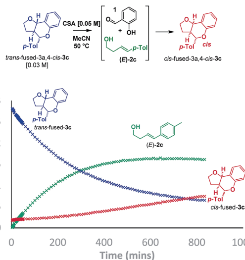
Scheme 6 Isomerization study by 1 H NMR.
