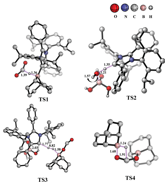
Fig. 8 Optimized structures of the transition states involved in the potential energy surface of \text{CO}_2 reduction to methoxyborane and sodium formate with 2 in air. Important bond distances (in Å) are shown. Only relevant H atoms are provided in the structures.
