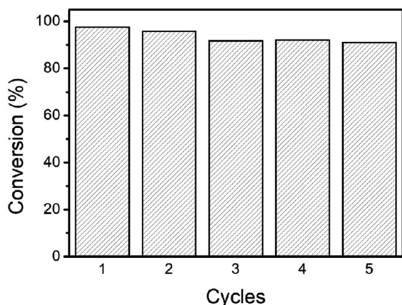
Fig. 7 The reusability of Ag/ZnO/CaCO 3 in the reduction of 4-NP with NaBH 4 .
