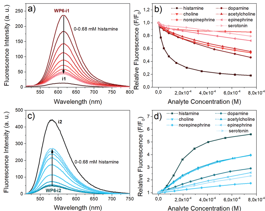
Fig. 6 Indicator displacement of the complexes with various neurotransmitter analytes in HEPES buffer (pH 7.4). (a) Fluorescence spectra of WP6·i1 (0.9 \mu M i1, 5.8 \mu M WP6, \lambda_{\text{ex}} : 482 nm) upon addition of histamine (0 to 0.68 mM) (b) relative fluorescence values of WP6·i1 at 615 nm upon addition of different analytes (c) fluorescence spectra of WP6·i2 (0.9 \mu M i1, 126 \mu M WP6, \lambda_{\text{ex}} : 438 nm) upon addition of histamine (0 to 0.68 mM) (d) relative fluorescence values of WP6·i2 at 533 nm upon addition of different analytes.
