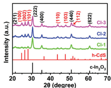
Fig. 1 XRD patterns of the as-prepared CdS/ \text{In}_2\text{O}_3 heterostructures.
