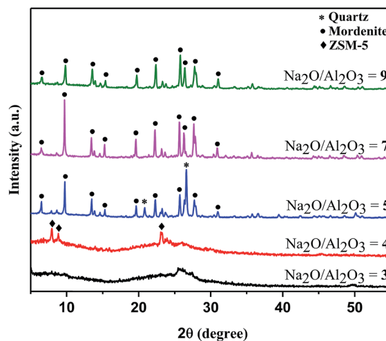
Fig. 4 XRD of samples synthesized from a reagent mixture of NaOH, \text{Na}_2\text{SiO}_3 , \text{Al}_2(\text{SO}_4)_3 , and \text{SiO}_2 ( \text{Na}_2\text{O} : \text{Al}_2\text{O}_3 : \text{SiO}_2 ratio of x : 1 : 30 , where x = 3 –9) that was mechanochemically ground for 50 min, then thermally treated at 180 °C for 48 h, and then washed with water. Peaks for \text{Na}_2\text{O}/\text{Al}_2\text{O}_3 ratio of 7 and 9 correspond to mordenite, at a ratio of 5 mordenite also contains weak quartz peaks near 22 and 27°, and at ratio of 4, weak ZSM-5 is present.
