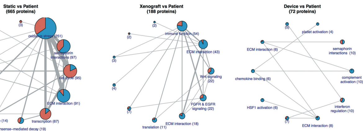
Fig. 8 The PDAC TMES is most similar to the patient transcriptome. Protein–protein interaction networks representing differential expression states between the patient biopsy and each culture condition. Each node represents collections of densely connected proteins ( i.e. , communities). The number of proteins in each community is proportional to the node size, and the proportion of up- (red) and down-regulated (blue) genes is encoded in the node color.
