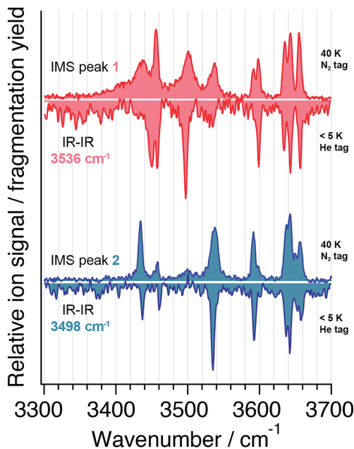
Fig. 4 IR spectra of two conformers of Gal \beta (1-4)GlcNAc acquired with the IR-IR double resonance method (downward pointing) with the pump laser fixed at 3536 cm -1 (red) and at 3498 cm -1 (blue), respectively. The spectra of the ion-mobility separated species 1 and 2 (upward pointing) are displayed for comparison in red and blue, respectively.
