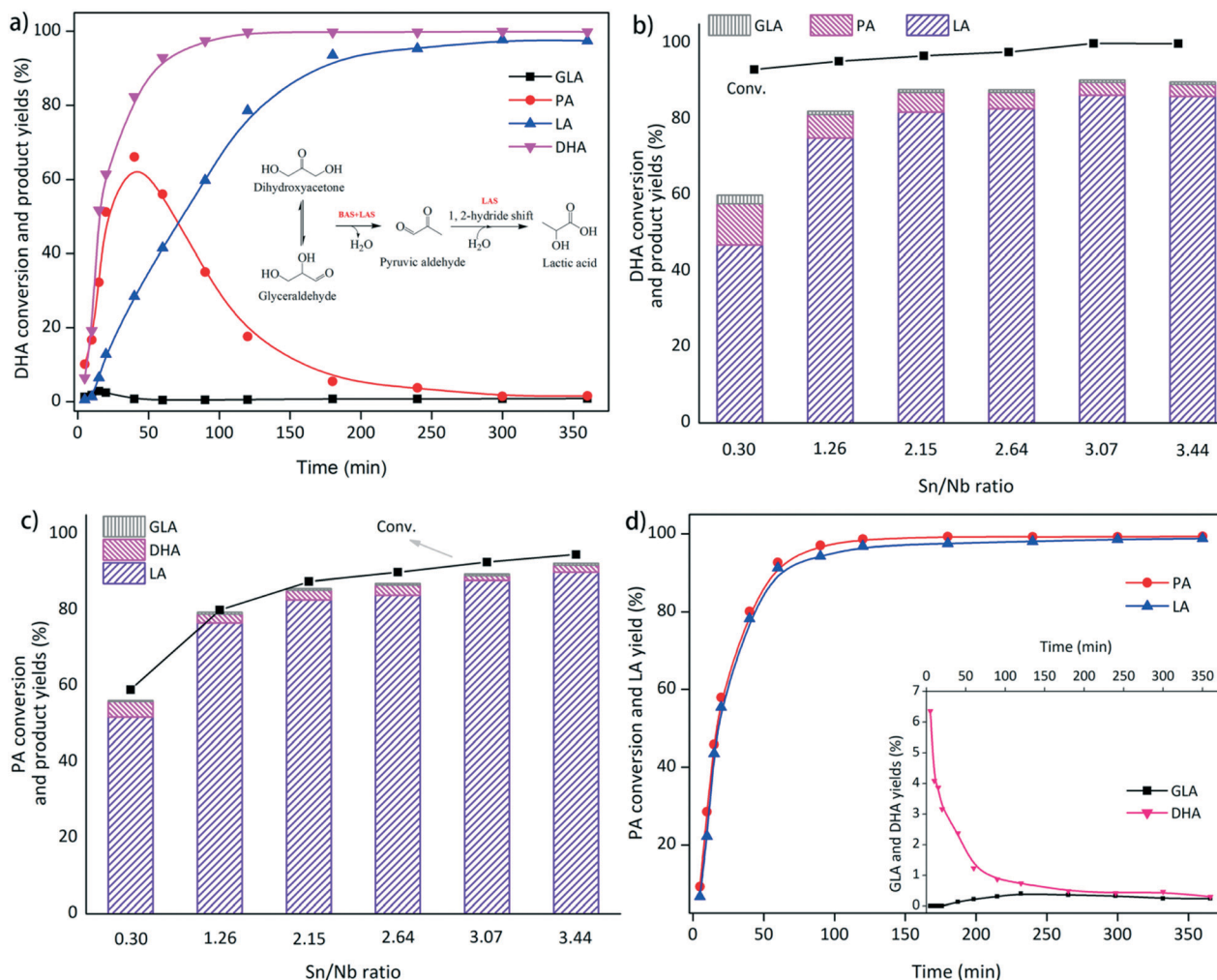
Fig. 5 a) Time evolution of the DHA conversion over \text{SnO}_2/\text{Nb}_2\text{O}_5 -3.07 ( [\text{DHA}]_0 = 0.2 M, catalyst = 50 mg, T = 120 °C. Inset: Reaction pathway). b) Conversion of DHA over \text{SnO}_2/\text{Nb}_2\text{O}_5 with different surface Sn/Nb ratios (the Sn/Nb ratios were determined by XPS analysis) ( [\text{DHA}]_0 = 0.2 M, catalyst = 50 mg, T = 140 °C, time = 1 h). c) Conversion of PA over \text{SnO}_2/\text{Nb}_2\text{O}_5 with different surface Sn/Nb ratios (the Sn/Nb ratios were determined by XPS analysis) ( [\text{PA}]_0 = 0.2 M, catalyst = 50 mg, T = 140 °C, time = 1 h). d) Time evolution of the PA conversion over the \text{SnO}_2/\text{Nb}_2\text{O}_5 catalysts ( [\text{PA}]_0 = 0.05 M, catalyst (Sn/Nb ratio = 3.07) = 50 mg, T = 140 °C).
