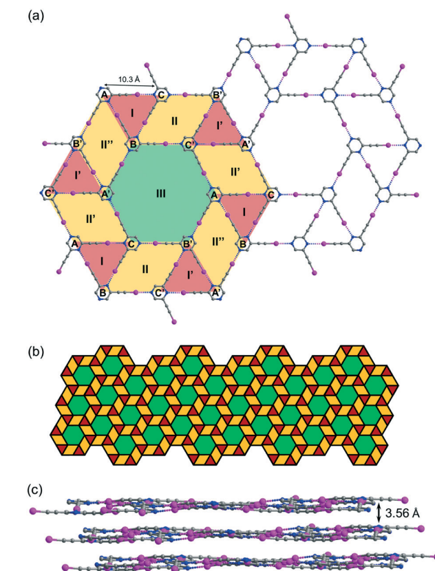
Fig. 5 (a) Projection diagram showing the tacit trihedral snub trihexagonal tessellation stabilized by C–I \cdots N halogen bonds with three independent L2 molecules in L2b. (b) Schematic diagram showing the pattern of the complete tessellation of a single layer in L2b. (c) Projection diagram showing the stacking of the tiling layers in the crystal structure. All hydrogen atoms are omitted for clarity.
