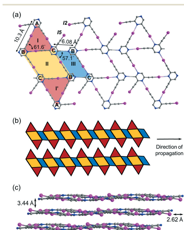
Fig. 4 (a) Projection diagram showing the triangle-rhombus-parallelogram ribbon constructed by C–I \cdots N halogen bonds and C–H \cdots N hydrogen bonds between three independent L2 molecules in crystal form L2a. (b) Schematic diagram showing two adjacent toothy-edged ribbons in a single layer in L2a. (c) Projection diagram along the a -axis showing the stacking of wavy tessellated layers. All hydrogen atoms are omitted for clarity.
