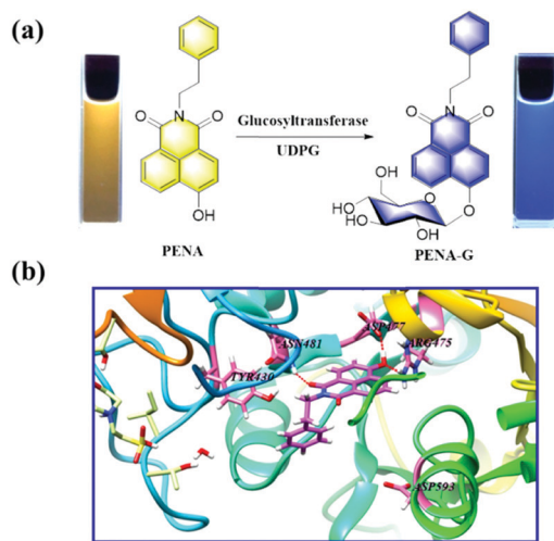
Fig. 1 (a) Glucosylation of PENA by GTFs in the presence of UDPG (300 \mu\text{M} ). (b) In silico docking analysis for the interaction between PENA and GTFs molecule.
