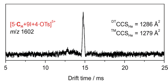
Fig. 7 DT-IM-MS ATDs of ions derived from pentameric halogen-bonded capsule 3. Experimental ^{DT}CCS_{He} and theoretical ^{TM}CCS_{He} values are given.
