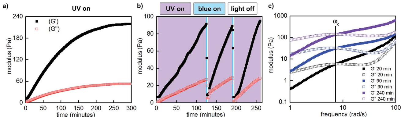
Fig. 5 Representative photorheological characterization of the hydrogels obtained at 25–28 °C. (a) UV-induced gelation profile of P1 and P2 (1 : 1, 10 w/v% in PBS, pH 7.5, 10% strain, 25 rad s −1 ). (b) Photocontrolled cycling of hydrogel viscoelasticity (10% strain, 25 rad s −1 ). UV light induces gelation, which is reversed with blue light. UV light is required to re-initiate stiffening of the gel. The first gelation cycle is slower than subsequent cycles; for a discussion, see the ESI.† (c) Dynamic frequency sweep measurements as a function of irradiation (10% strain).
