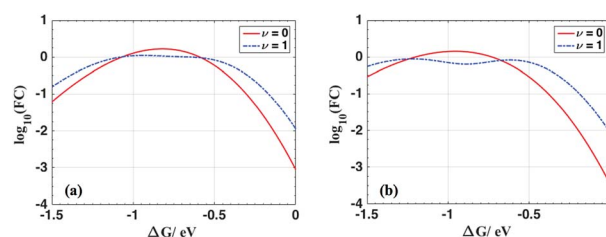
Fig. 5 Plot of \log_{10}(\text{FC}_{\nu=0}) (red solid lines) and \log_{10}(\text{FC}_{\nu=1}) (blue dotted lines) as a functions of \Delta G for \lambda_o = 0.7 eV and (a) S = 1 ; (b) S = 2 at room temperature with \hbar\omega = 1200 cm -1 . The ET rate is predicted to decrease in the near activationless regime ( \Delta G + \lambda_i + \lambda_o - \hbar\omega \approx 0 ) due to IR excitation of the quantum reaction coordinate and to increase elsewhere.
