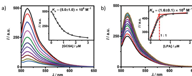
Fig. 1 (a) Direct fluorescence titration of Fl (1.0 \mu M ) with GC5A (up to 3.0 \mu M ), \lambda_{em} = 500 nm. (Inset) the associated titration curve at \lambda_{em} = 513 nm and the fit according to a 1 : 1 binding stoichiometry. (b) Competitive titration of GC5A·Fl (0.4/0.5 \mu M ) with LPA (up to 1.9 \mu M ). (Inset) fit of the titration data to a 1 : 1 competitive binding model. All experiments are in HEPES buffer (10 mM, pH = 7.4) at 25 °C.
