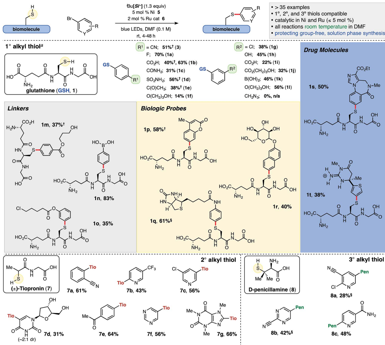
Chart 1 Ni/Photoredox thioarylation reaction and scope of various thiol and arene small molecules. ^t\text{Bu}[\text{Si}^-] = diisopropylammonium bis(catechol)isobutylsilicate. DMF = N,N -dimethylformamide. Reactions conducted with 0.1 mmol thiol and ArBr, unless otherwise noted; isolated yields are reported (TFA salt omitted for clarity, see ESI† for additional details). a 0.12 mmol GSH employed. § 2 equiv. ArBr was employed. † The adduct was filtered following precipitation from the aqueous solution.
