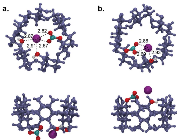
Fig. 6 Top and side views of the optimized structures of the ionic alkyl carbonate at α-CD: (a) Reaction at the primary C-6 position. (b) Reaction at the secondary C-2 position.
