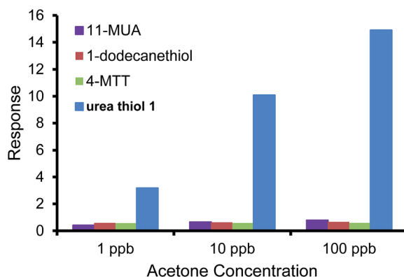
Fig. 6 The responses of sensors derived from AuNPs coated with urea thiol 1, 1-dodecanethiol 4-methoxy- \alpha -toluenethiol (4-MTT) and 11-mercaptopundecanoic acid (11-MUA) in detection of a mixture of 1 ppb benzene, 1 ppb ethanol and acetone varied from 1 ppb to 100 ppb.
