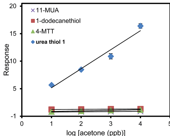
Fig. 5 Responses for sensors derived from AuNPs coated with urea thiol 1, 1-dodecanethiol, 4-methoxy- \alpha -toluenethiol (4-MTT) or 11-mercaptopundecanoic acid (11-MUA) in detection of acetone.
