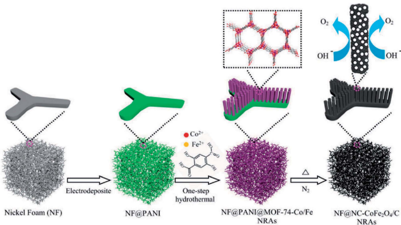
Fig. 8 Schematic representation of one-step PANI-assisted synthesis of a bimetal–organic framework NRAs and its derived porous \text{CoFe}_2\text{O}_4/\text{C} NRAs. Reproduced with permission from ref. 149. Copyright 2017 Wiley.
