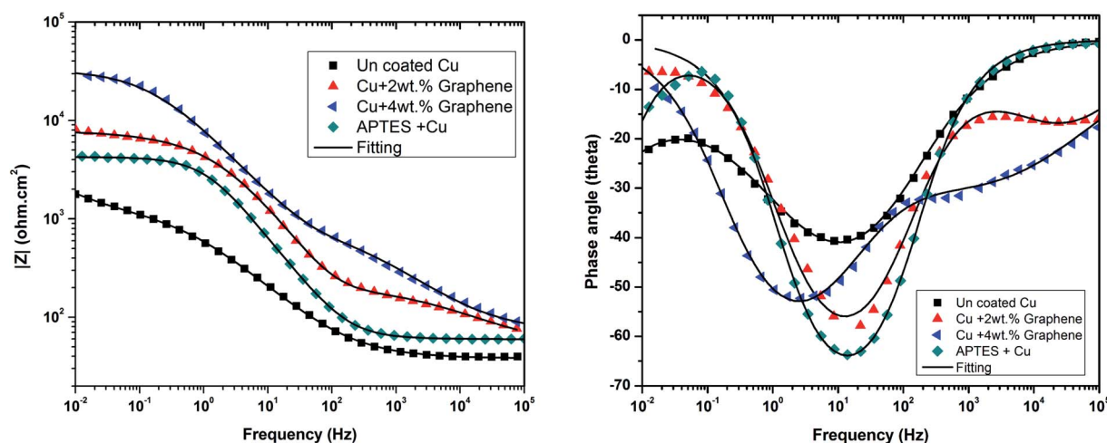
Fig. 8 Electrochemical impedance plots obtained in 3.5 wt% NaCl at OCP.
