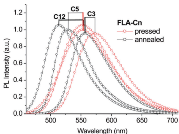
Fig. 6 (Top) The molecular structure of compound 12 . (Bottom) Emission spectra of FLA-C n solids mixed with KBr upon pressing and annealing. Reproduced with permission from ref. 35. Copyright 2013 The Royal Society of Chemistry.
