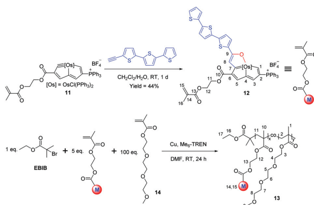
Scheme 2 Synthesis of osmapentalenofuran 12 with the methacrylate group and metallopolymer 13 .
