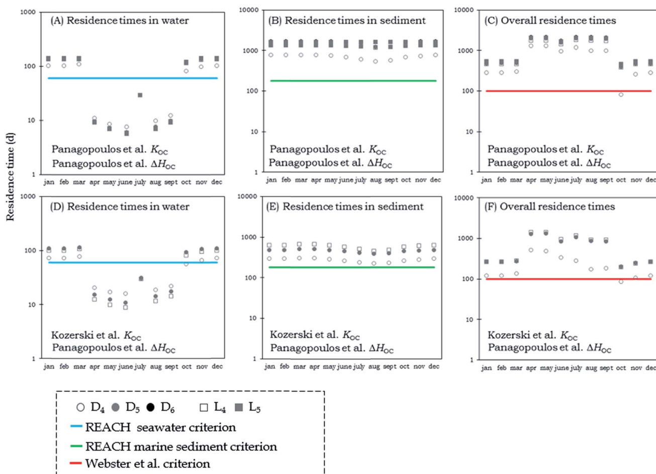
Fig. 4 Water, sediment and overall residence times for cVMS (circles) and lVMS (squares) using both the K_{OC} measurements of Kozerski et al. 26 (lower panels) and those of Panagopoulos et al. 16,17 (upper panels). The K_{OC} was corrected for temperature changes using the \Delta H_{OC} measurements of Panagopoulos et al. 32 The blue line shows the REACH criterion for persistence in marine waters and the green line shows the REACH criterion for persistence in marine sediments. 24 The red line shows the 100-day overall persistence criterion suggested by Webster et al. 25
