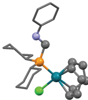
Fig. 4 X-Ray structure of (\text{C}^6\text{Hex}_2\text{PCH}_2\text{NHPh})\text{Rh}(\text{cod})\text{Cl} [CCDC 748467]. 51
