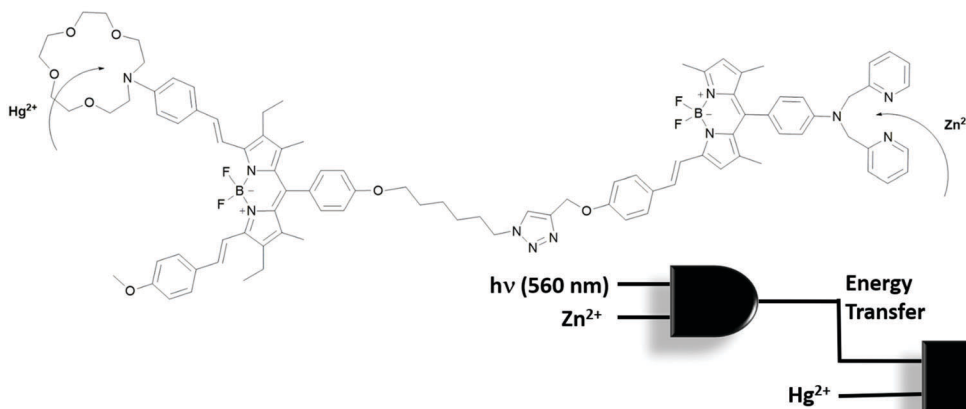
Fig. 10 Structures of physically integrated AND logic gates and their logic diagrams.
