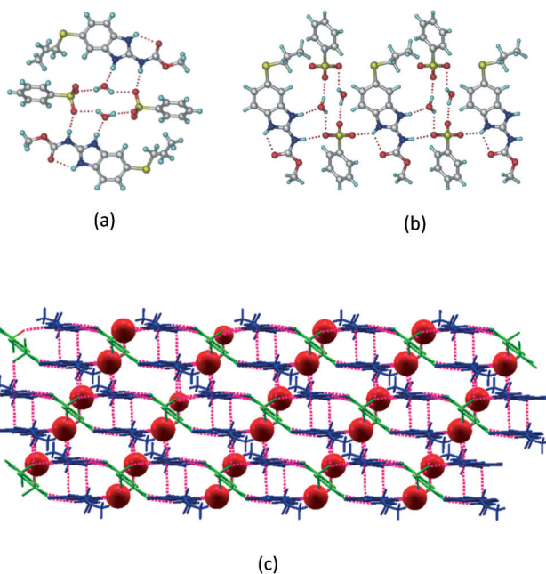
Fig. 3 (a) The bridging water molecules act as proton donors for the sulfonate and acceptors for N + -H resulting in the ring network R_3^2(8) R_4^4(12)R_3^2(8) . (b) The sulfonate-water molecules are bonded via N-H...O - hydrogen bonds to ABZ. (c) Complete packing of cations, anions and water molecules.
