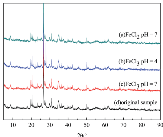
Fig. 11 The XRD spectra of the arsenic waste slag samples obtained before and after the stabilization step was carried out using \text{FeCl}_2 and \text{FeCl}_3 .
