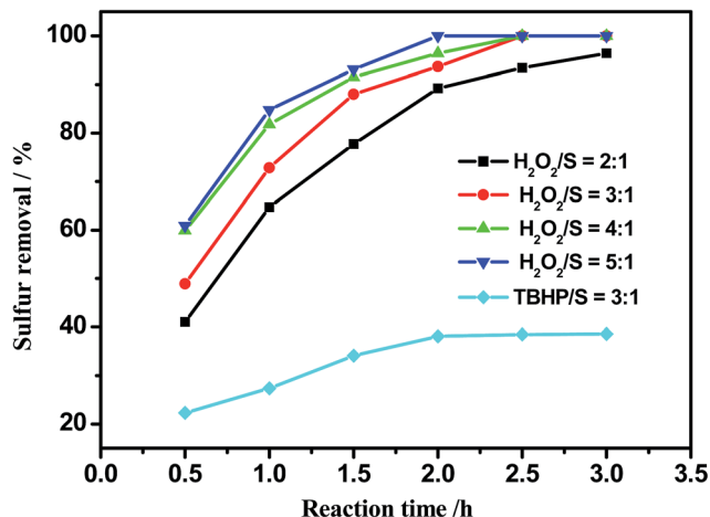
Fig. 4 Effect of the oxidant on sulfur removal. Experimental conditions: m(\text{catalyst}) = 0.025\text{ g} , ChCl/2Ac = 2 mL, oil = 5 mL, T = 40\text{ }^{\circ}\text{C} .
