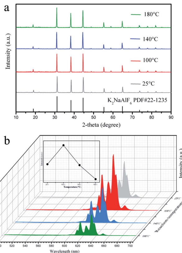
Fig. 6 (a) XRD patterns and (b) emission spectra ( \lambda_{\text{ex}} = 460 nm) of the \text{K}_2\text{NaAlF}_6\text{:Mn}^{4+} samples synthesized at different reaction temperatures.
