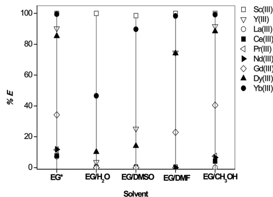
Fig. 10 Influence of addition of polar solvent (50% (v/v)) to ethylene glycol on the solvent extraction of REEs. EG* = EG feed without added polar solvent. Experimental conditions: [RE(III)] : \sim 2.5 \text{ g L}^{-1} (each), [LiCl] : 2 \text{ M} , [Cyanex 923] : 1 \text{ M} in n -dodecane with 10% (v/v) 1-decanol.
