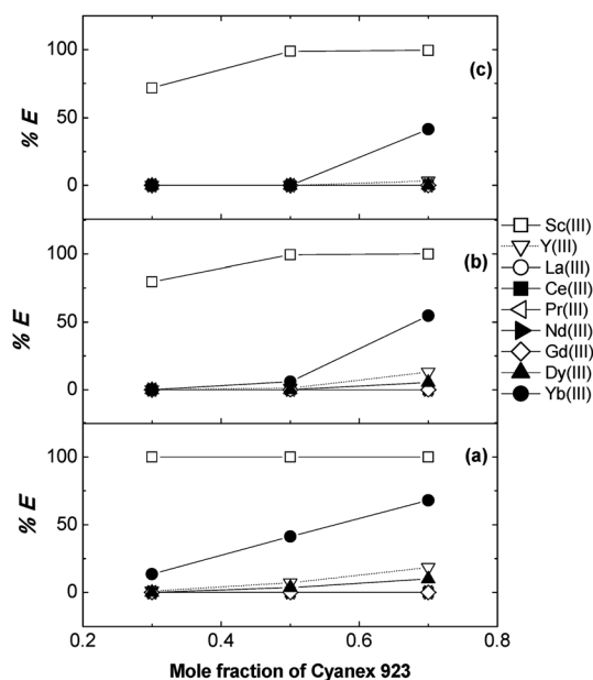
Fig. 9 Solvent extraction of REEs from ethylene glycol (+LiCl) solutions using a mixture of Cyanex 923 and Cyanex 272 (a), TBP (b), Aliquat 336 (c) in n -dodecane. Experimental conditions: [RE(III)] : \sim 5 \text{ g L}^{-1} (each), [LiCl] : 2 \text{ M} , [Cyanex 923 + \text{other extractant}] : 1 \text{ M} .
