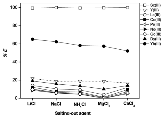
Fig. 8 Influence of the source of chloride ions on the solvent extraction of REEs. Experimental conditions: [RE(III)] : \sim 5 \text{ g L}^{-1} (each), [Cl^-] = 1 \text{ M} , [Cyanex 923] : 1 \text{ M} in n -dodecane with 10% 1-decanol (v/v).
