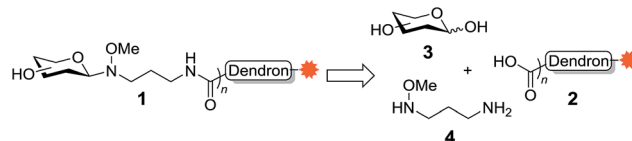
Scheme 1 Assembly of glycodendrons using an amine-functionalised oxyamine linker.
