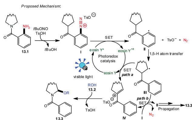
Scheme 13 Oxidative synthesis of \alpha -alkoxybenzamides.
