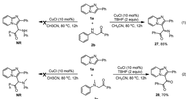
Scheme 2 Selective coupling of imidazopyridine 1a with \alpha -amino phenylethanone.
