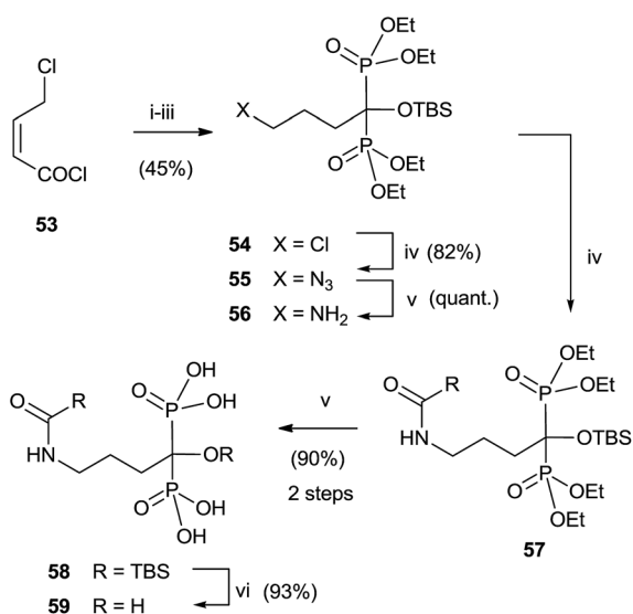
Scheme 10 Reagents and conditions: (i) \text{P}(\text{OEt})_3 , 0 °C. (ii) \text{HOP}(\text{OEt})_2 , DMAP, \text{CH}_2\text{Cl}_2 , room temp, 1 h. (iii) TBSCl, 15 h. (iv) \text{NaN}_3 , DMF, 75 °C, 2 h. (v) Pd-C, 50 psi of \text{H}_2 , AcOEt, 15 h. (vi) \text{RCOCl} , \text{Et}_3\text{N} , \text{CH}_2\text{Cl}_2 or \text{RCO}_2\text{H} , EDC, DIPEA, MeCN. (v) TMSI, MeCN and then MeOH. (vi) TBAF, THF.
