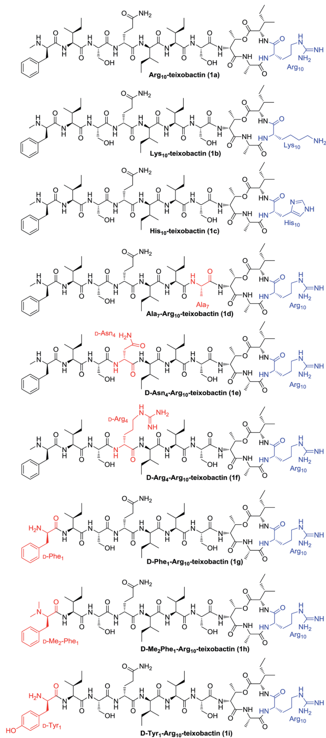
Fig. 2 Structures of teixobactin analogues 1a–i .
