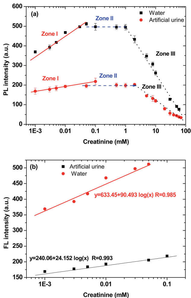
Fig. 3 (a) FL intensities at 375 nm with creatinine concentration in water and artificial urine and (b) zone I region in water and artificial urine. \lambda_{\text{ex}} = 262 \text{ nm} ; [IDATPE] = 40 \mu\text{M} ; measured at t = 5 \text{ min} .
