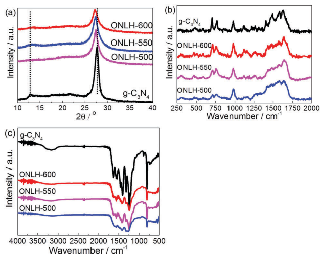
Fig. 2 Characterization of ONLH and g-C 3 N 4 : (a) powder XRD pattern, (b) Raman spectra (325 nm excitation), and (c) FT-IR spectra.
