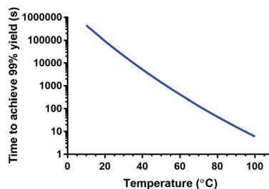
Fig. 6 Prediction of time needed to achieve 99% yield for [^{177}\text{Lu}]\text{Lu-DOTA-TATE} in a setup with optimal heat and mass transfer. The graph was calculated using the Arrhenius parameters obtained in this study.
