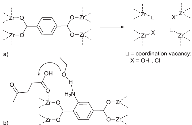
Fig. 30 (a) Defect formation through a missing linker. Two Zr atoms have a vacancy and two Zr ions from different \{Zr_6\} clusters are coordinated by hydroxido or chlorido anions in order to retain framework neutrality. (b) Proposed reactivation pathway over UiO-66-NH 2 . Redrawn from ref. 155. Copyright 2015 with permission from Elsevier.
