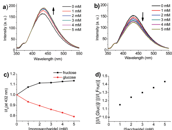
Fig. 4 (a) Fluorescence spectra of 1.33 \times 10^{-6} M sensor 14 upon addition of fructose (0–5 mM) in pH 8.21 methanolic buffer; (b) fluorescence spectra of 1.33 \times 10^{-6} M sensor 14 upon addition of glucose (0–5 mM) in pH 8.21 methanolic buffer; (c) plotting fluorescence responses of 14 against the concentrations of fructose and glucose; (d) plot of [(I/I_0) \text{ Gluc}]/[(I/I_0) \text{ Fruc}] against the concentration of tested saccharide. Excitation wavelength: 330 nm; maximum emission: 432 nm.
