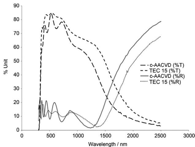
Fig. 13 Optical transmittance (%T) and reflectance (%R) spectra of SnO 2 :F lab-grown by combinatorial aerosol-assisted chemical vapour deposition (c-AACVD) as compared with an industrial SnO 2 :F product (TEC 15, Pilkington NSG). Adapted with permission from Bhachu et al. 37 Copyright 2011 Wiley.
