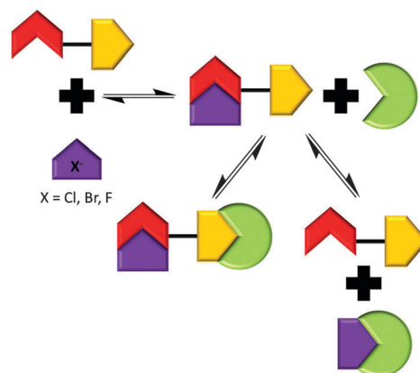
Scheme 5 Summary of the proposed hydrogen bonded complexes formed from solutions of 1 with combinations of 6 and competitive anionic guests in \text{DMSO} , based on the NMR evidence presented herein.
