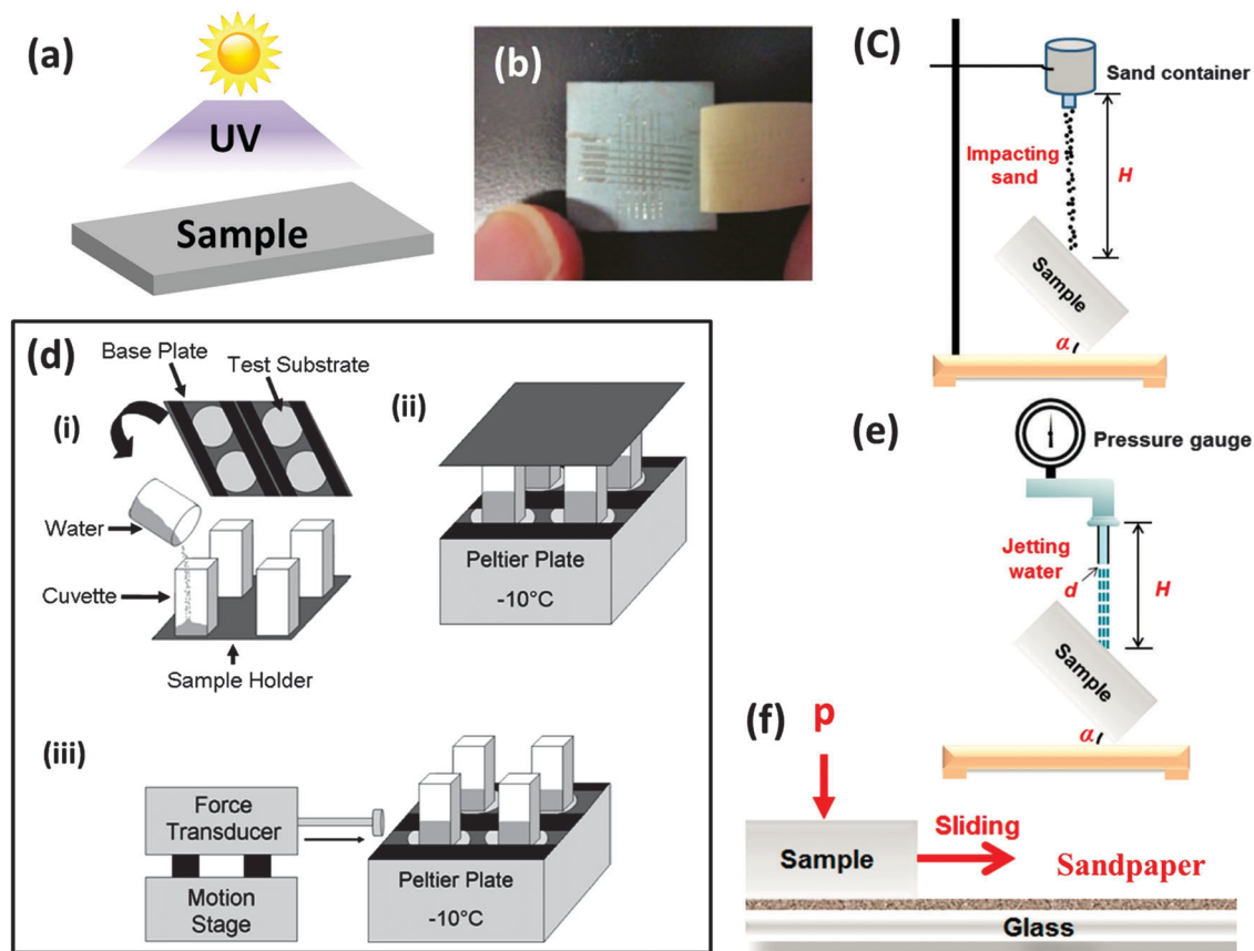
Fig. 9 Common methods in use to quantify the durability of the superhydrophobic/icephobic surfaces. (a) UV irradiation, (b) tape adhesion test, 127 (c) sand impact test, 112 (d) ice formation/ice removal cycles 3 (e) water jet/dripping test 112 and (f) sandpaper abrasion measurement. 112 Other common durability tests are immersion in salt solution or organic solvent, ultra-sonication, pencil hardness test, wipe test, and thermal treatment. (Not shown in the figure) Figures reproduced from ref. 3, 112 and 127 with permission from ACS, Elsevier, and ACS, respectively.
