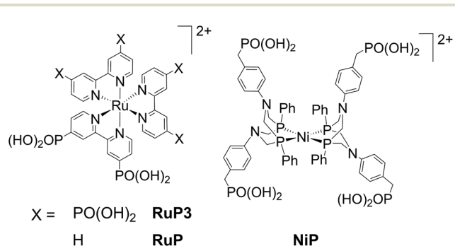
Fig. 1 Structures of the dyes ( RuP and RuP3 ) and proton reduction catalyst ( NiP ) used in this study. Chloride ( RuP3 ) and bromide ( RuP , NiP ) counter-ions are omitted for clarity.
