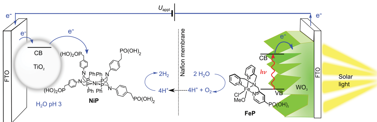
Scheme 1 Schematic representation of PEC water splitting with the TiO 2 | NiP hydrogen evolution cathode wired to the WO 3 | FeP oxygen evolution photoanode in an aqueous electrolyte solution at pH 3.
