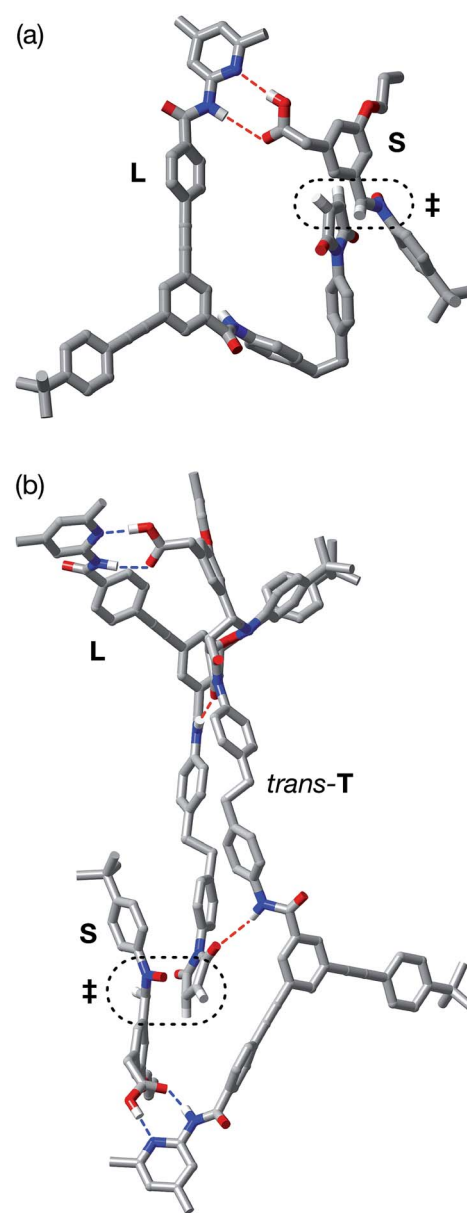
Fig. 10 (a) Stick representation of the computed transition state geometry (RM1) leading to the formation of trans -T' formed through the [L·S] complex. (b) Stick representation of the computed transition state geometry (RM1) leading to the formation of [trans-T·trans-T] through the ternary complex [L·S·T]. Carbon atoms are coloured grey, nitrogen atoms are coloured blue, oxygen atoms are coloured red and hydrogen atoms are coloured white. For clarity, most hydrogen atoms are not shown. Hydrogen bonds with D–H⋯A distances <2.0 Å are shown as blue dashed lines, hydrogen bonds with D–H⋯A distances between 2.0 and 2.5 Å are shown as red dashed lines. The transition states for the forming isoxazolidine rings are enclosed in the black dotted lines.
