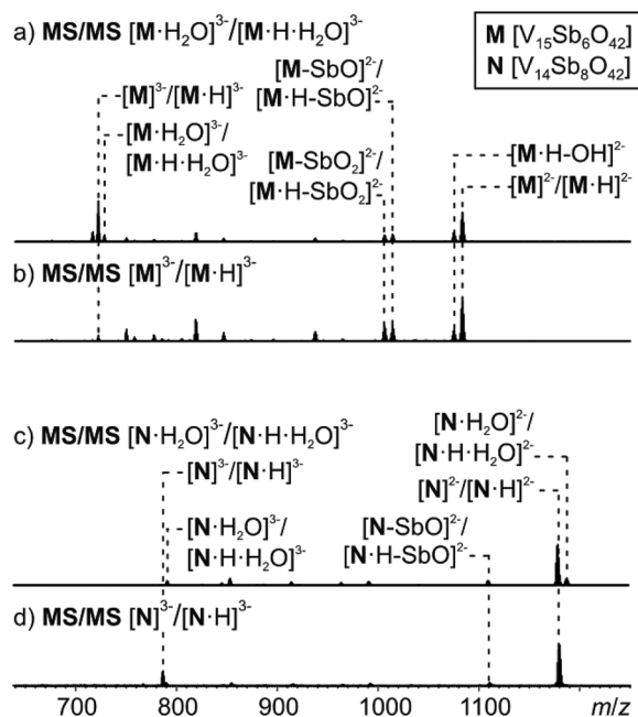
Fig. 8 Tandem MS experiment of (a) complex [\mathbf{M} \cdot \text{H}_2\text{O}]^{3-} , (b) complex \mathbf{M}^{3-} , (c) complex [\mathbf{N} \cdot \text{H}_2\text{O}]^{3-} , (d) complex \mathbf{N}^{3-} .
