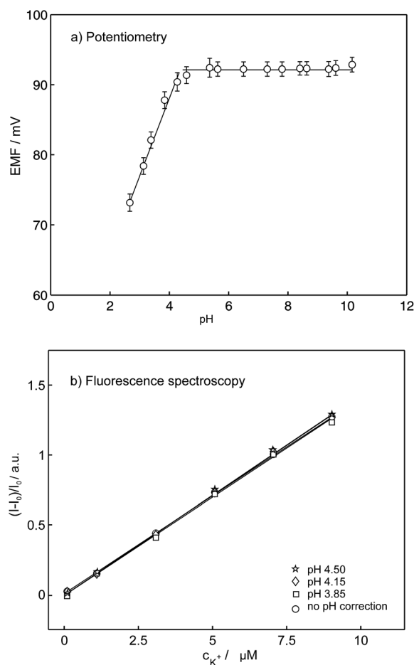
Fig. 9 (a) Potentiometric response of the potassium selective sensor to the changes in concentration of H^+ at fixed concentration of potassium 1 mM and (b) observed linear calibration curves from the normalized fluorescence spectra as a function of potassium concentration at different pH.
